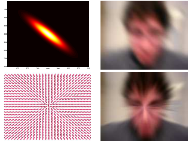
Figure 1: Behavior of trace-based PDE's (6) (right) with constant or spatially varying tensors \mathbf{T} (respectively top and bottom left).
