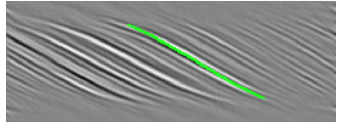
Figure 6. Result of fiber tracking on front and back layers of the composite (green line).
