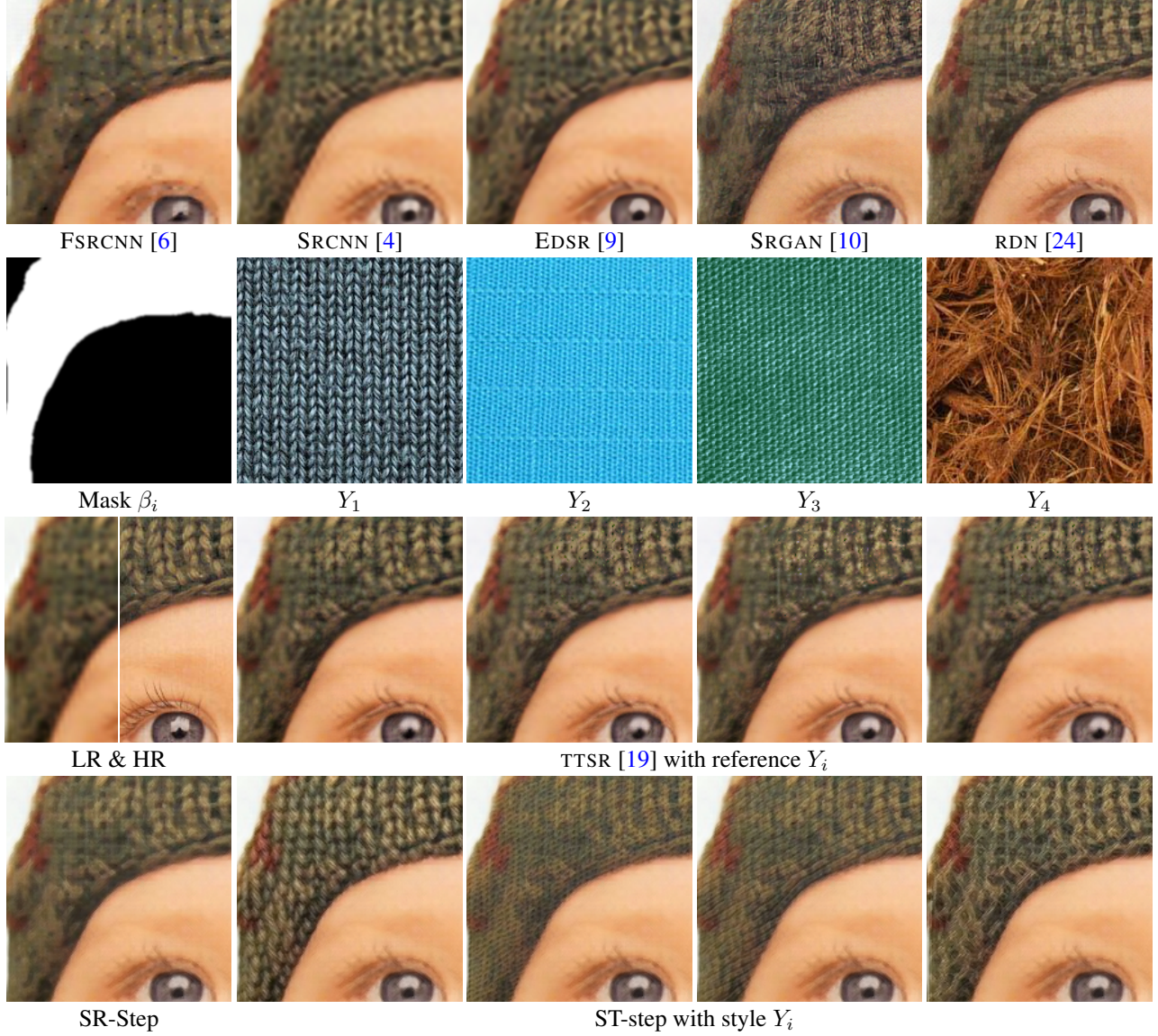
Fig. 3: Comparison of 4 \times SR results on cropped baby (Set5 dataset) for various SISR methods (first row) and RefSR methods (TTSR on third row, and proposed on fourth) with different styles Y_i (on second row). More examples can be found at [3].
